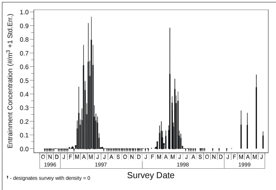
Figure 3-6. Weekly mean larval concentrations of kelp, gopher, and black-and-yellow (KGB) rockfish complex larvae at the Diablo Canyon Power Plant intake entrainment stations. Dark bars represent mean concentration and thinner bars represent one standard error.
