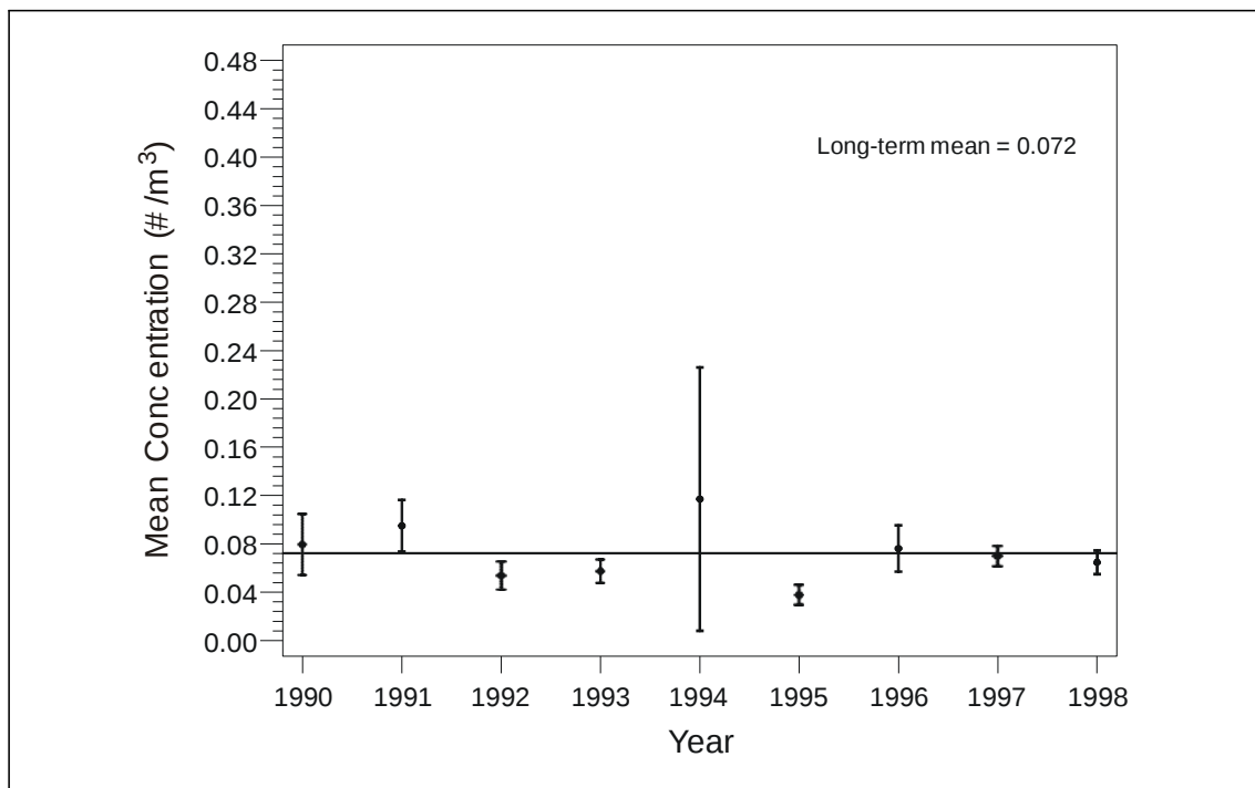
Figure 3-7. Annual mean concentration ( \pm 2 standard errors) for kelp, gopher, and black-and-yellow (KGB) rockfish complex larvae collected from surface plankton tows in DCPP Intake Cove. Data were collected from December through June for every year except 1990 when only data from February through June were collected. The horizontal line is the long-term mean for all years combined.
