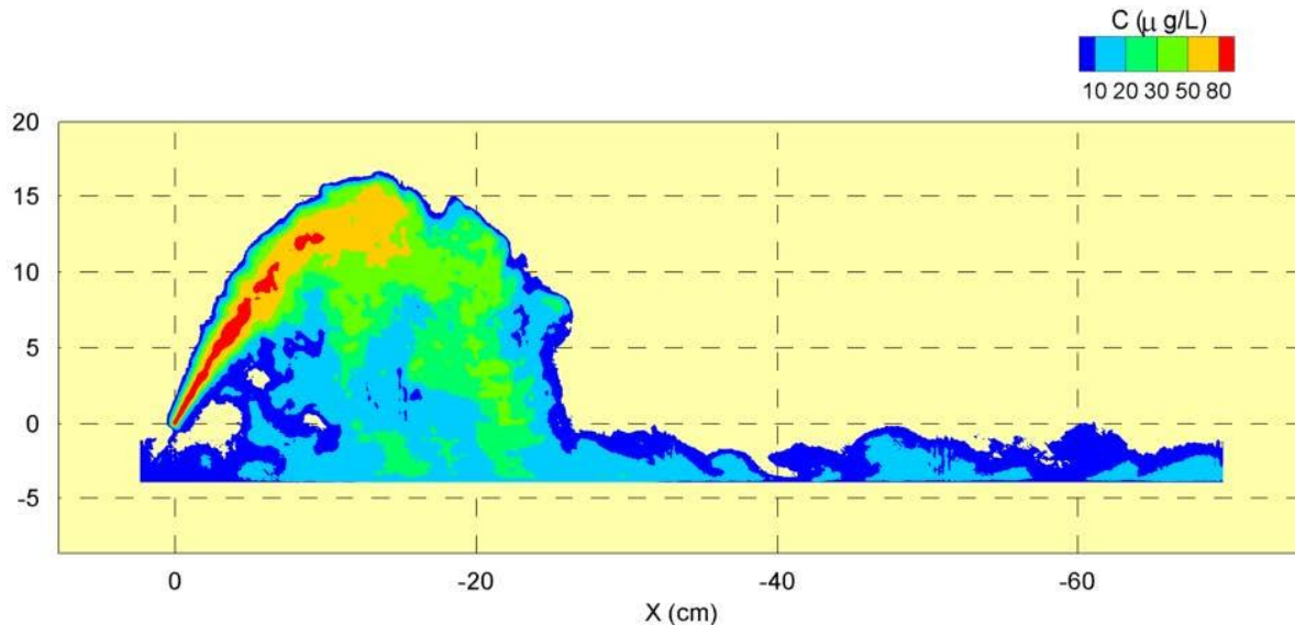
Figure 8-4. Laser-induced fluorescence animation image of a brine plume discharge from a diffuser. (From Roberts 2013)
